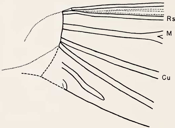
Fig. 3. Drawing of base of holotype forewing of Cretatermes carpenteri , new genus, new species, showing visible veins emerging from the humeral suture.
